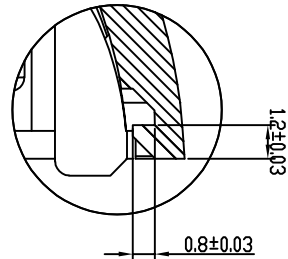
DETAIL D SCALE 5:1
